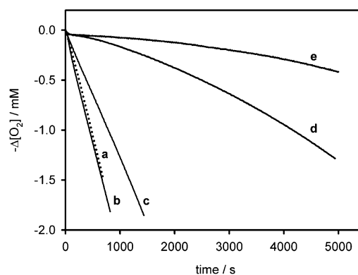
Figure 2. \text{O}_2 consumption during the autoxidation of styrene (4.3 M) in acetonitrile initiated by AIBN (0.05 M) at 30 °C (a, dotted line) and corresponding experiments carried out in the presence of 13 \mu\text{M} of either \text{TEMPO}^+\text{BF}_4^- (b,d) or TEMPO (c,e) with (d,e) or without (b,c) acetic acid (43 mM).
