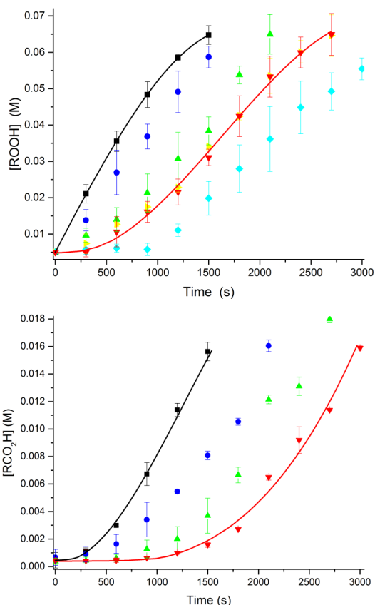
Figure 6. Hydroperoxide (top) and acid (bottom) formation in the autoxidation of light paraffin oil at 160 °C initiated by 5 mM tetralin hydroperoxide (black) and inhibited by 40 μM 2 (red) with 4 mM palmitic acid (yellow), 40 mM palmitic acid (light blue), 4 mM 2,4,6-( t -Bu) 3 pyridine (green), or 40 mM 2,4,6-( t -Bu) 3 pyridine (dark blue).
