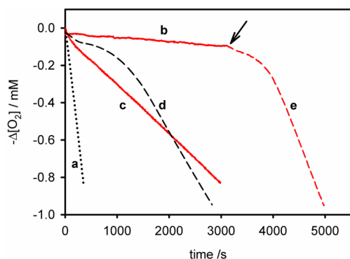
Figure 5. O 2 consumption during the autoxidation of styrene (4.3 M) in acetonitrile containing 1% H 2 O initiated by AIBN (0.05 M) at 30 °C (a) and corresponding experiments carried out in the presence of TEMPO (13 μM) and acetic acid (43 mM) (b), acetic acid (43 mM) and Oct 4 NBF 4 (0.13 M) (c), acetic acid (43 mM) and HBF 4 (43 mM) (d), and acetic acid (43 mM) with HBF 4 (43 mM) added at the time indicated by the arrow (e).
