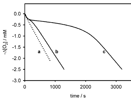
Figure 3. O 2 consumption during the autoxidation of styrene (4.3 M) in chlorobenzene initiated by AIBN (0.05 M) at 30 °C (a, dotted line) and corresponding experiments carried out in the presence of 13 μM of either TEMPO + BF 4 - (b) or TEMPO (c) and AcOH (44 mM).
