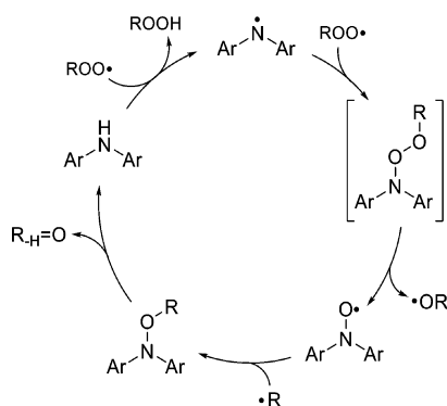
Scheme 6. Proposed Mechanism of Catalytic Activity of Diarylamine RTAs
