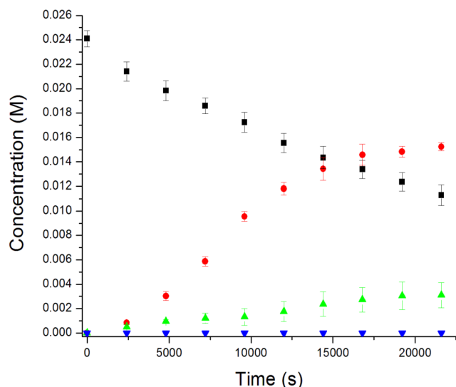
Figure 1. Decomposition of azocumene (black) and formation of the cumyl-TEMPO adduct in the presence of \text{TEMPO}^+\text{BF}_4^- (25 mM) and \text{Me}_4\text{N}^+\text{AcO}^- (25 mM) in acetonitrile at 50 °C under an atmosphere of argon (red), air (green) or \text{O}_2 (blue).
